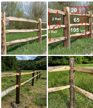
Cleft Split Chestnut Post & Rail Fencing, with 2 or 3 mortice posts
